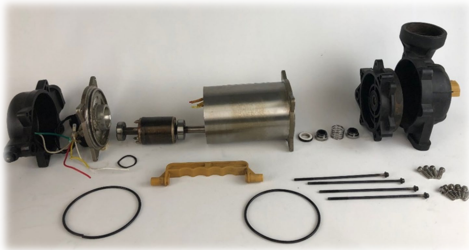
Direct Drive Pump
